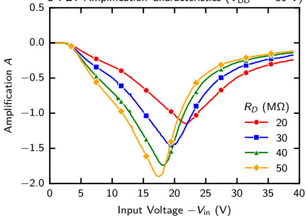
O-FET Amplification Characteristics ( V_{DD} = -30\text{ V} )
